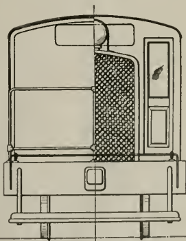
GENERAL ARRANGEMENT OF SIX-COUPLED, 15 AND 25 TON LOCOMOTIVE.
